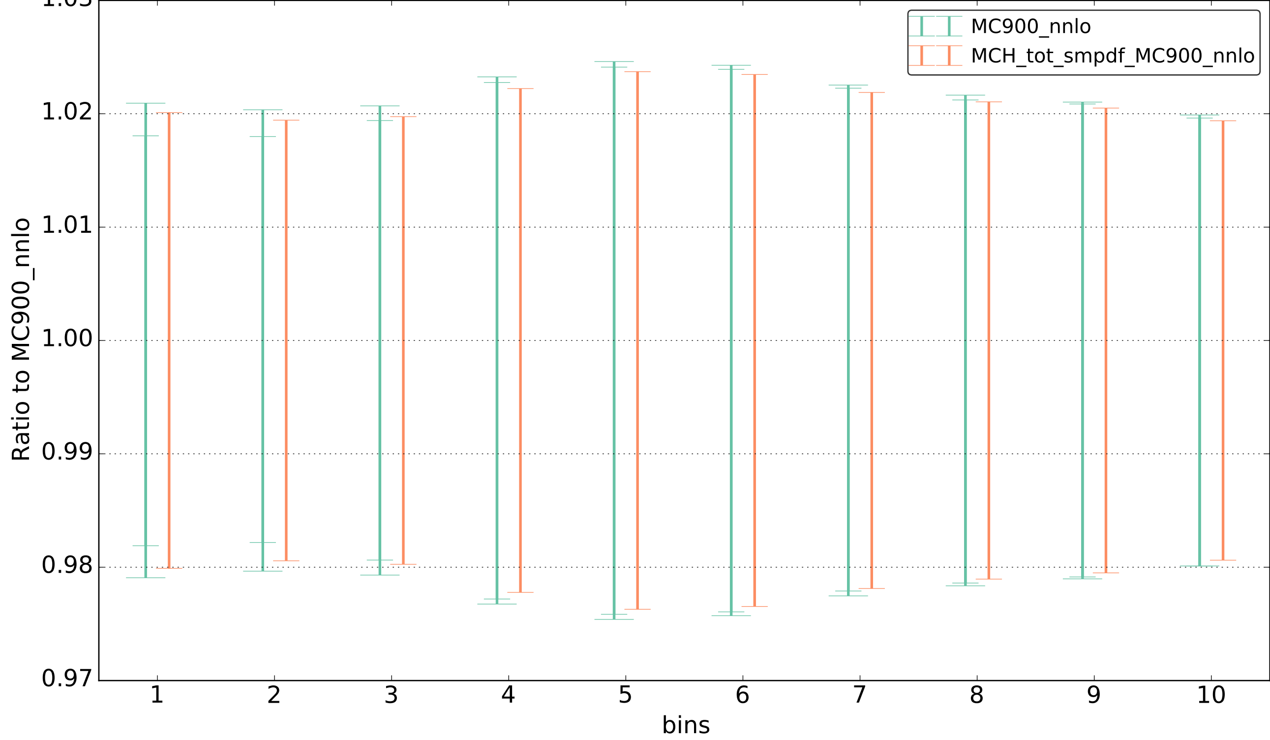
z_lplminvmass_13tev(NLO)
