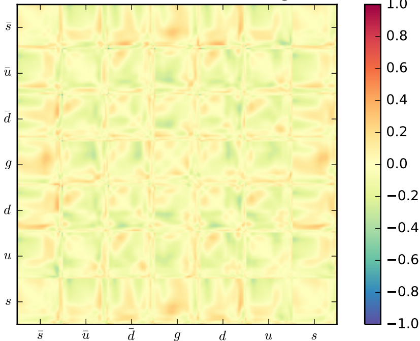
Correlations CMC70-MC900 NLO @ 8 GeV
